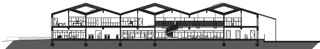
Section Aa
